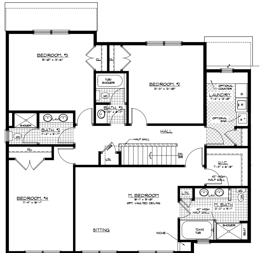
SECOND FLOOR
